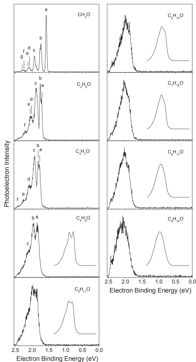
Fig. 1. Photoelectron spectra of the linear C_nH_{2n+1}O^- alkoxydes where n = 1–9 taken with 2.54 eV photons. Franck-Condon fittings are shown for n = 4–9 in the insets.
